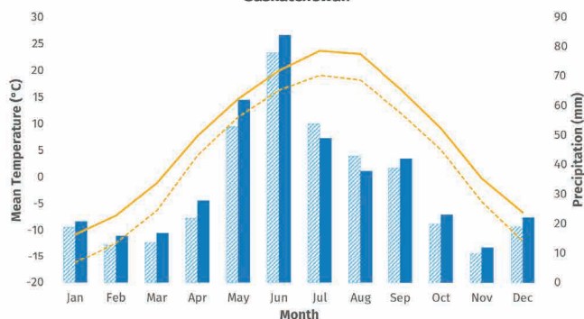
High-Carbon Climate Change Projections for Regina, Saskatchewan
